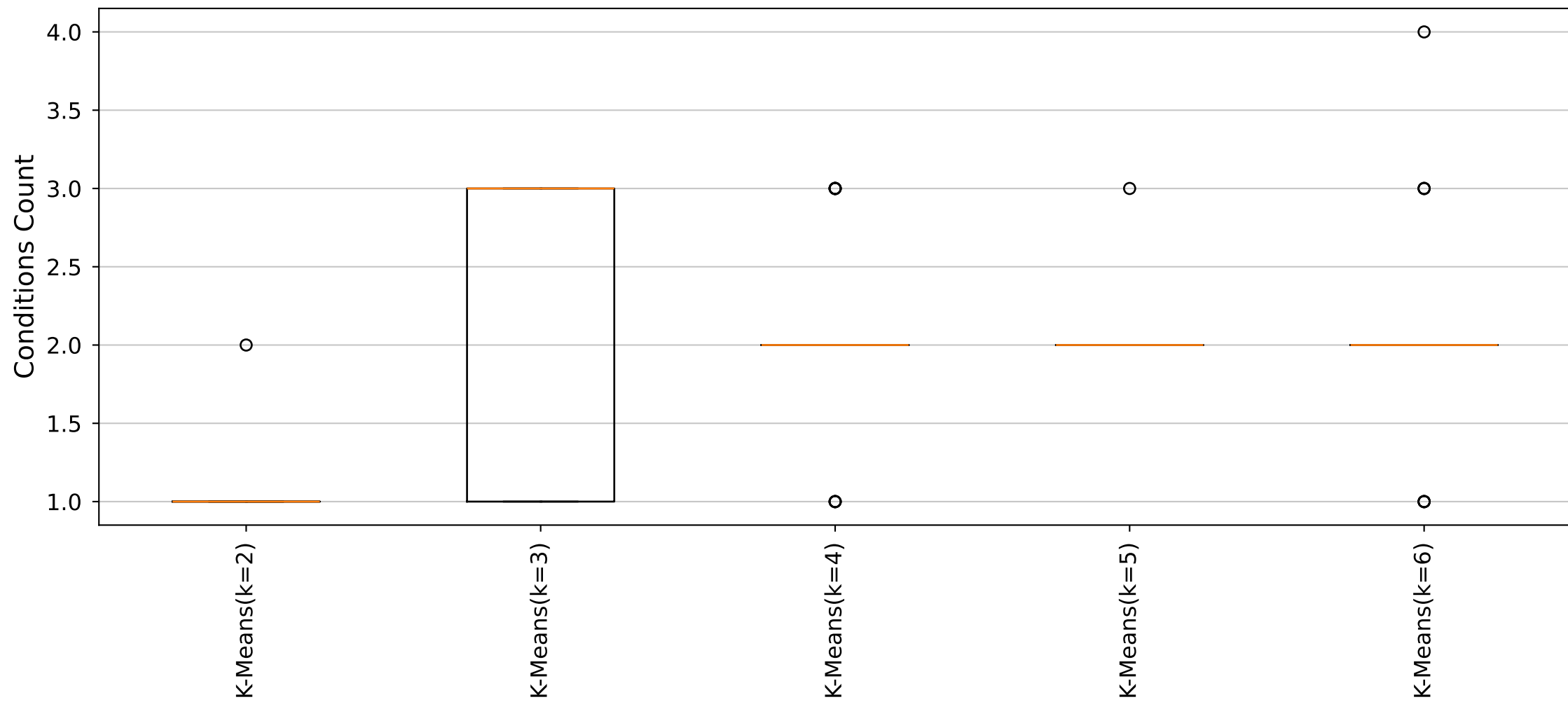
YARA Rules Conditions Count Distribution (Cluster32_Size6 dataset)
